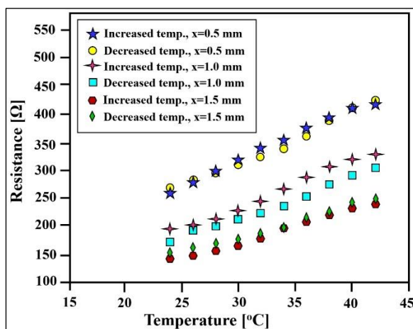
Fig. 10. Electrical resistance values vs. the temperature increased and decreased values for different central area thicknesses (Each point in the graph is an average of three measurements)
