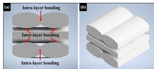
Fig. 2. Visualization of the PLA-BC raster 0^{\circ}/90^{\circ} building configuration unit cell (CAD model), showing the welding between the polymeric fibers located at the same layer (intra-layer weld), and the weld between two adjacent layers (inter-layer weld): (a) front view; and (b) isometric view [7]
