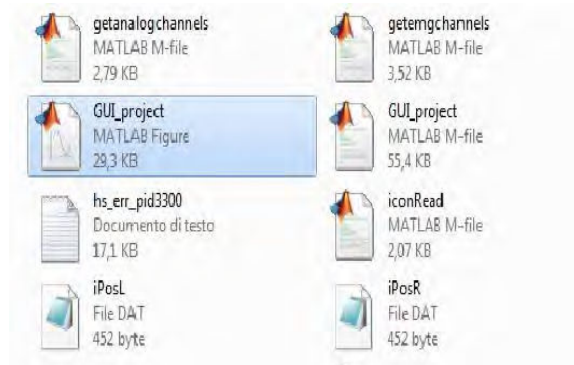
Fig.2. File GUI_project
