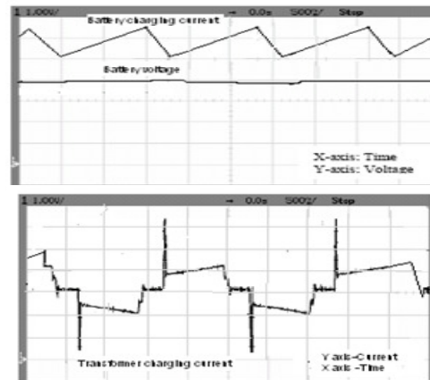
Fig.8. Battery charging current battery voltage and transformer charging current waveforms in forward mode operation
