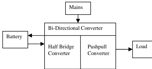
Fig.2. Figure 2. Block diagram of proposed converter
