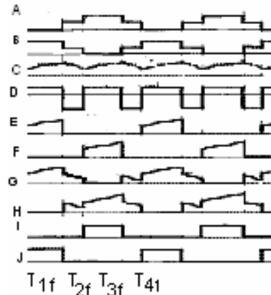
Fig.4. Waveforms during forward mode operation A)Voltage across switch S1 B)Voltage across switch S2 C)Load current D)Load Voltage E)Current through S1 F)Current through S2 G)Current through body diode of S3 H)Current through body diode of S4 I)Voltage across switch S4 J)Voltage across switch S3
