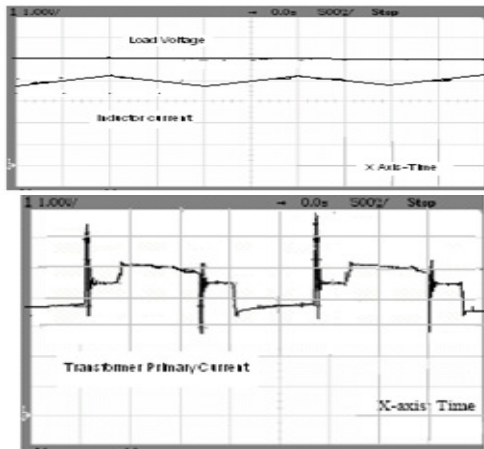
Fig.9. Back up mode Load voltage, inductor current, transformer primary current
