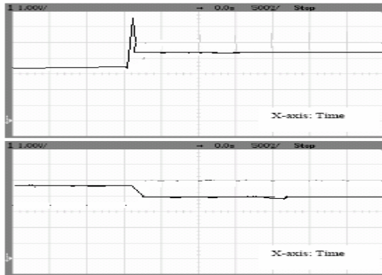
Fig.9. Back up mode Load voltage, inductor current, transformer primary current
