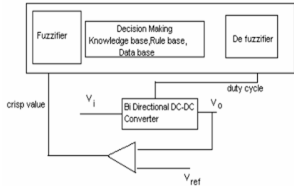
Fig.1. Block diagram of Fuzzy logic Controlled Converter.
