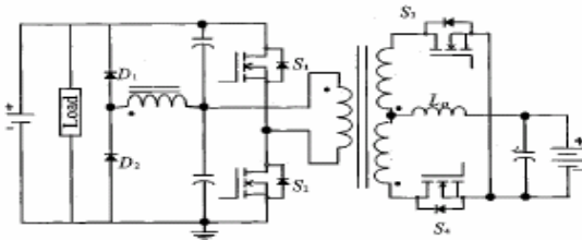
Fig.3. Power Circuit of Proposed Converter
