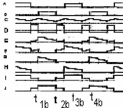
Fig.5. Waveforms during backup mode operation
