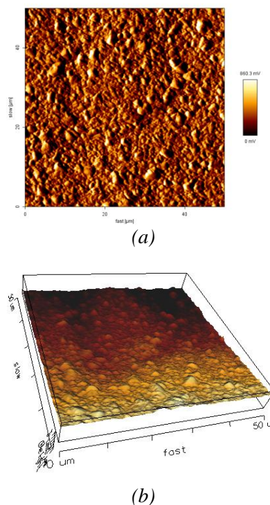
Fig. 1. AFM images of pure nickel surface electrodeposited at 2A/dm 2 : 2D (a) and 3D (b)
