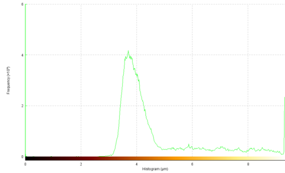
Fig. 8. Histogram of the scanned surfaces for Ni / micro-SiC composite layers obtained at 4A/dm^2
