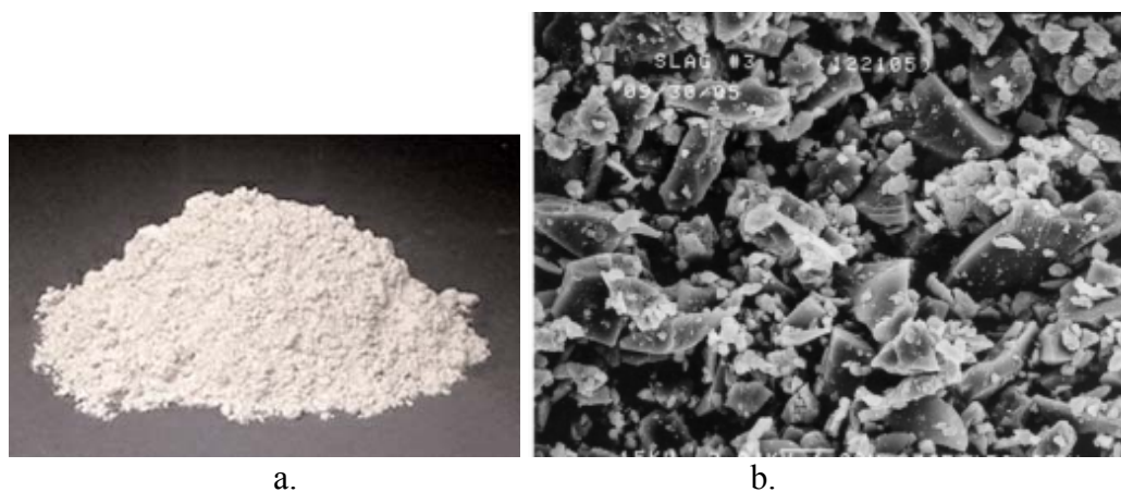
Fig. 8. Ground granulated blast-furnace slag (a) and its SEM micrograph (b) [16]
