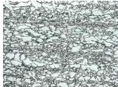
Fig. 8. Intercritical thermomechanical treatment state - D variant (x500).
