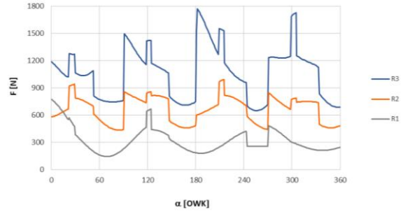
Fig. 15. Reaction values in camshaft bearings as a function of the rotational angle, for its average rotational speed of 2000 rpm and belt tension of 200 N
