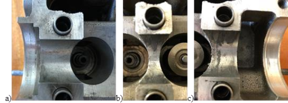
Fig. 19. Appearance of worn bearing bushings of camshaft slide bearings on the cylinder head side, a) bearing 3, b) bearing 2, c) bearing 1
