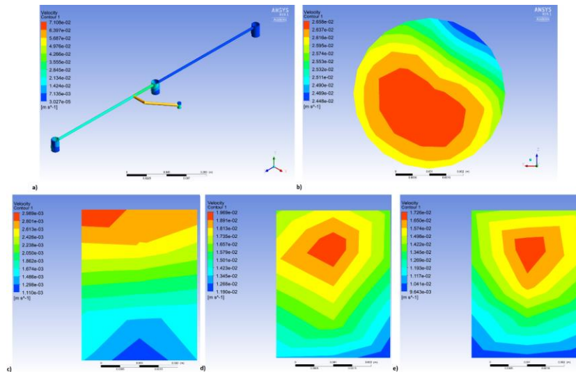
Fig. 11. Distributions of oil flow velocity for the boundary condition on the inflow in the form of a constant pressure of 400 kPa a) for the oil main line, b) at the inlet, c) at the Outlet1, d) at the Outlet2, e) at the Outlet3.
