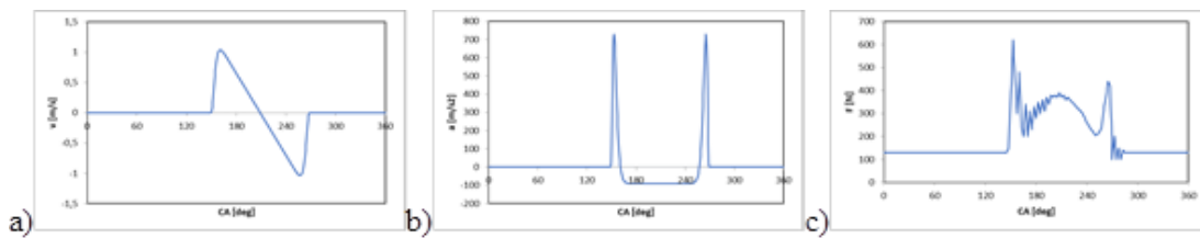
Fig. 12. Waveforms of a) speedy, b) acceleration of the tappet, c) force F acting on the tappet as a function of the rotational angle of the camshaft
