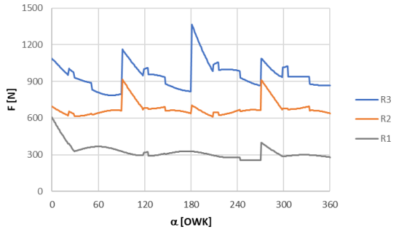
Fig. 13. Reaction values in camshaft bearings as a function of the rotational angle for its average rotational speed of 750 rpm and belt tension of 200 N
