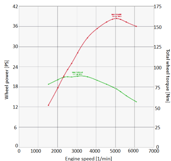
Fig. 1. Exemplary waveforms of measured engine power and torque as a function of engine speed for the engine SI R4 1.2 8V FIAT Punto II 2005
