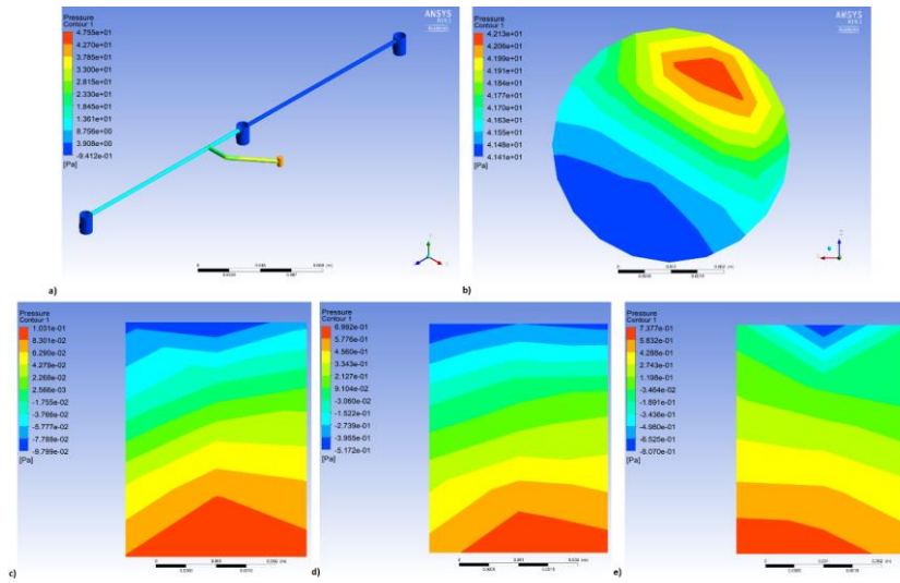
Fig. 10. Distribution of oil pressure for the boundary condition at the inflow in the form of a constant pressure of 400 kPa, a) for the oil main line, b) at the inlet, c) at the Outlet1, d) at the Outlet2, e) at the Outlet3
