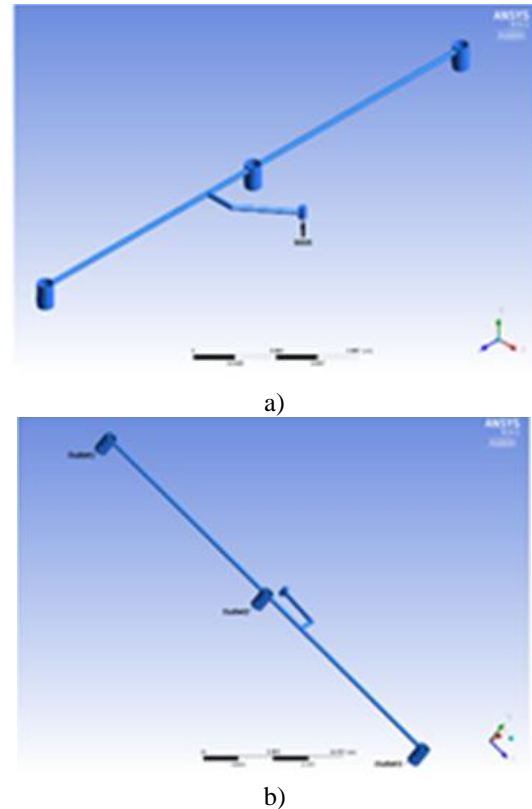
Fig. 4. Model of the controlled oil volume. a) (Inlet) - place of oil supply to the channel in the cylinder head, b) (Outlet1, Outlet2, Outlet3) - oil outlets into friction contact zones in camshaft bearings, c) finite element mesh
