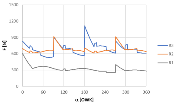
Fig. 14. Reaction values in camshaft bearings as a function of the rotational angle for its average rotational speed of 750 rpm and belt tension of 50 N
