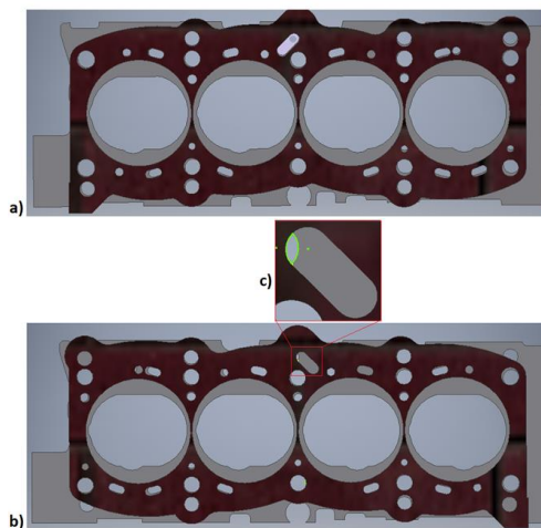
Fig. 5. Arrangement of the gasket relative to the head, a) correct, b) incorrect, c) enlarging the view of the pocket before entering the oil main line for camshaft bearings
