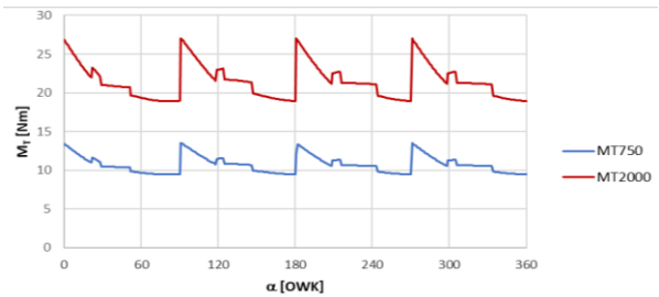
Fig. 18. The technically dry friction torque in camshaft bearings as a function of its rotational angle, for two values of camshaft rotational speed equal to 750 rpm and 2000 rpm
