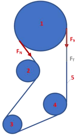
Fig. 7. Forces from the toothed belt loading the timing pulley. 1 - toothed pulley on the camshaft, 2 - tensioner, 3 toothed pulley on the crankshaft, 4 - toothed pulley on the water pump shaft, 5 - toothed belt. F_N - force from the toothed belt tension, F_T - force resulted from the part of the driving torque on the engine crankshaft.
