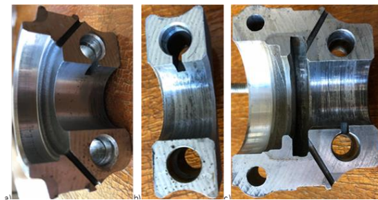
Fig. 20. Appearance of worn bearing bushings of cam roller bearings on the side of bearing covers, a) bearing 3, b) bearing 2, c) bearing 1
