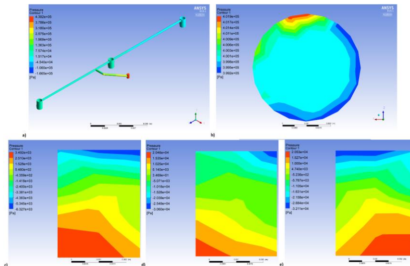
Fig. 9. Oil pressure distribution for the boundary condition on the inlet in the form of mass flow 0.00035 kg/s, a) for the oil main line, b) at the inlet, c) at the Outlet1, d) at the Outlet2, e) at the Outlet3
