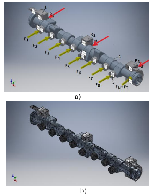
Fig. 6. a) The model of the tappets-camshaft-bearings assembly, b) Finite element grid. 1, 2, 3 - bearing covers with fixed surfaces located on the plane containing camshaft bearings axles, 4 - cam shaft, 5 - tappet with fixed axis of rotation, F_1, F_2, F_3, F_4, F_5, F_6, F_7, F_8 - forces loading the consecutive tappets mating with the shaft cams 4, F_N - force from the toothed belt tension, F_T - force resulted from the part of the drive torque acting on the toothed pulley mounted on the camshaft, R_1, R_2, R_3 - reactions in bearings 1, 2, 3
