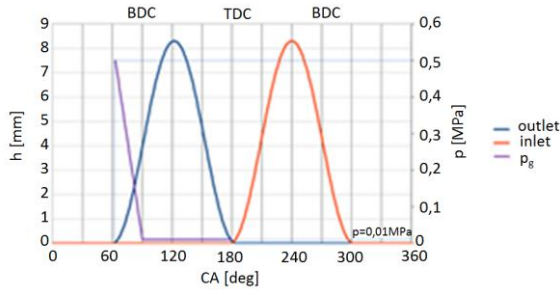
Fig. 2. The graph of valve lifts and modelled pressure p_g in the cylinder as a function of camshaft rotation for the engine SI R4 1.2 8V FIAT Punto II 2005
