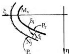
Fig. 6. Effective profile of cutting edge (approximated profile)
