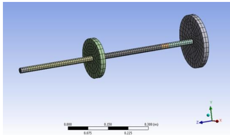
Fig. 4. System mesh - 8484 nodes and 1549 elements
