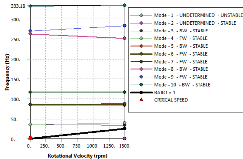
Fig. 6. Campbell diagram of the system with Fly-wheel
