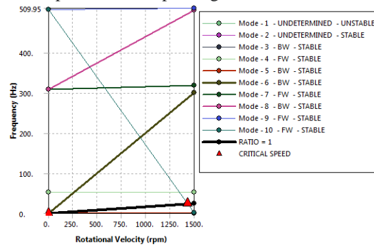
Fig. 7. Campbell diagram of the system without Fly-wheel
