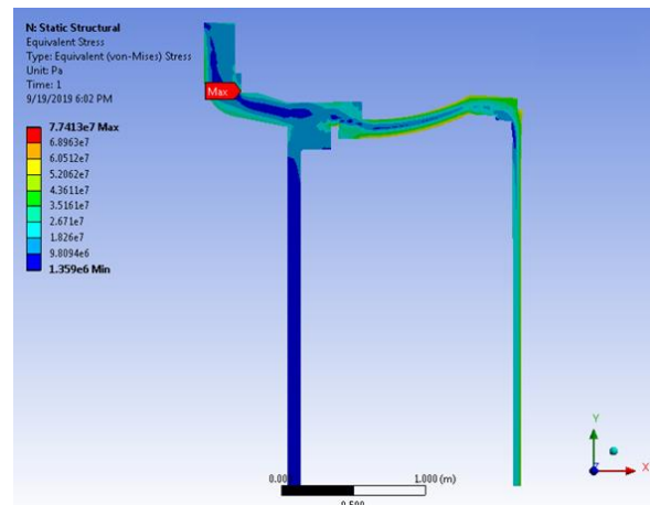
Fig. 14.a. Distribution of von Mises stresses for the 20 mm crack case in Zone 1 (ensemble)
