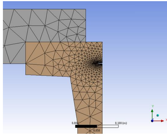
Fig. 6. Discretization around the crack in Zone 1 (20mm length)
