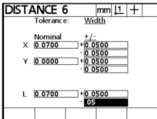
Fig. 8 Establishing allowable tolerances [3]
