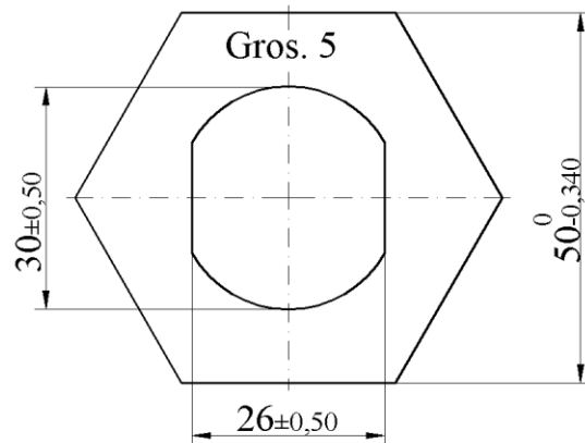
Fig. 2. Washer drawing [3]
