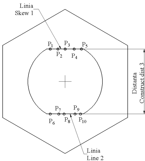
Fig. 7. Establishing a new alignment and building distance
